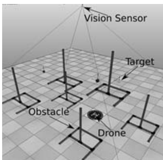
Figure 4: V-REP scene for Task 1.2
